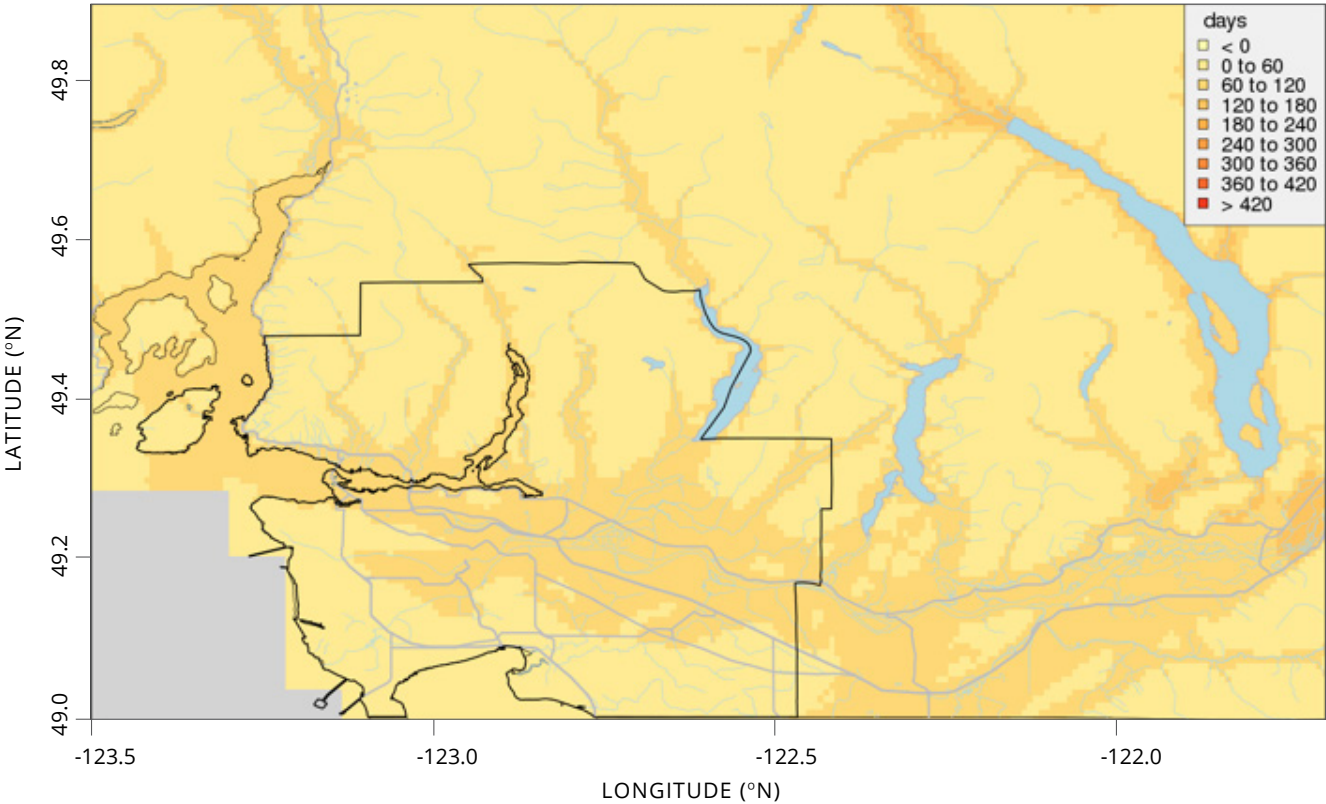
FIGURE 15: COOLING DEGREE DAYS – PAST
