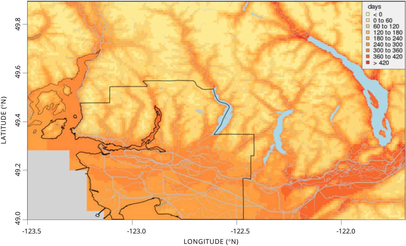
FIGURE 16: COOLING DEGREE DAYS – FUTURE (2050s)
