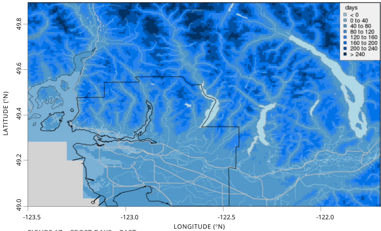
FIGURE 17: FROST DAYS – PAST
