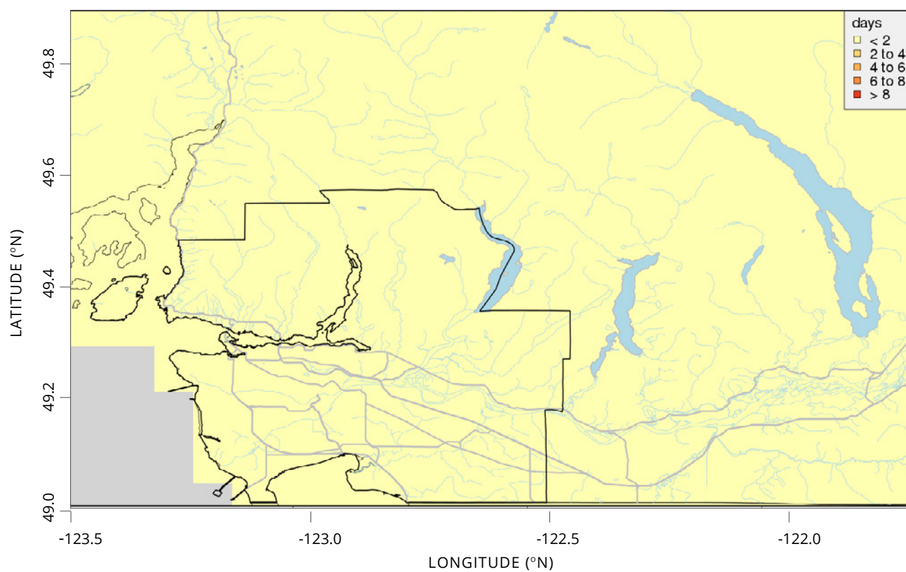
FIGURE A18: TROPICAL NIGHTS - PAST
