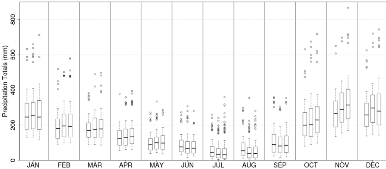
FIGURE A5 MONTHLY TOTAL PRECIPITATION FOR RCP4.5 Boxes from left to right in each month indicate past, 2050s, 2080s. Further explanation of how to read the box-and-whisker plots is provided above in the Methodology section.
