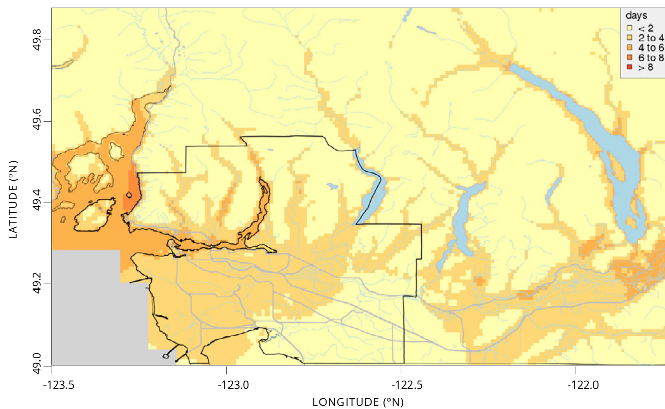
FIGURE A19: TROPICAL NIGHTS - FUTURE (2050s)
