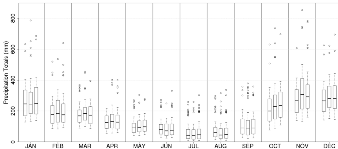
FIGURE A6 MONTHLY TOTAL PRECIPITATION FOR RCP2.6
